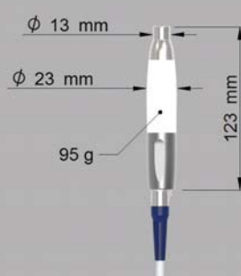
MUN.PZL - Led version
